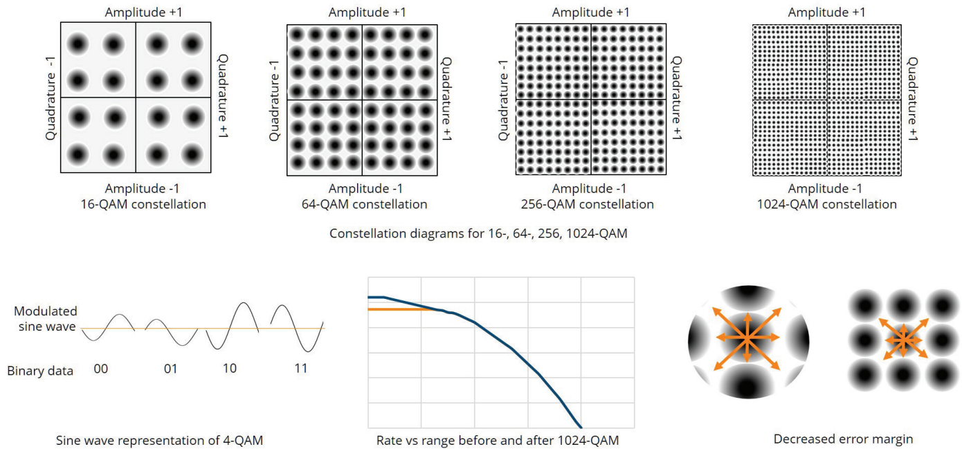
Figure 26: 1024-QAM modulation
