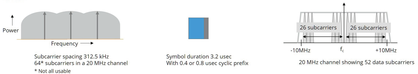
Figure 7: OFDM symbol duration &amp; subcarriers
