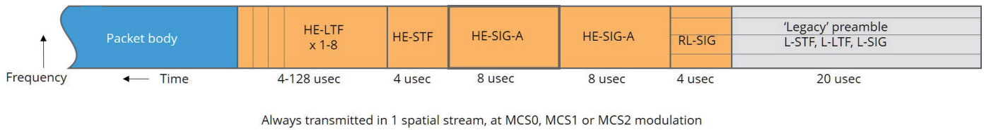
Figure 42: Single-user extended-range frame
