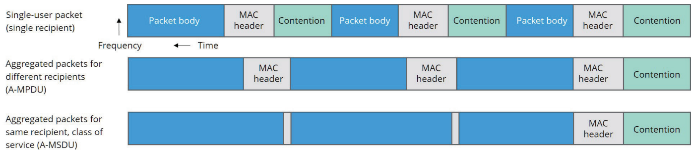
Figure 18: MAC Aggregation
