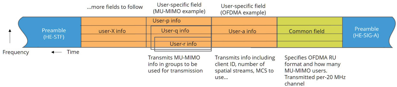
Figure 19: Control for multi-user downlink modes
