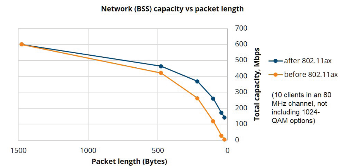
Figure 33: Network (BSS) capacity vs packet length
