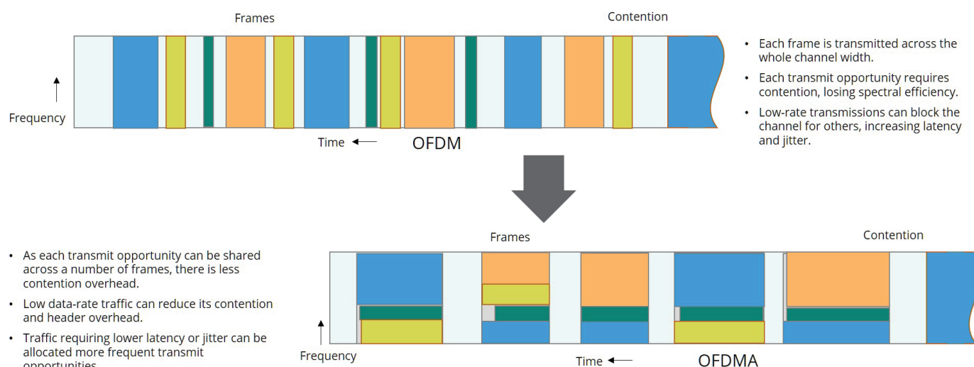
Figure 8: OFDMA compared with single-user OFDM
