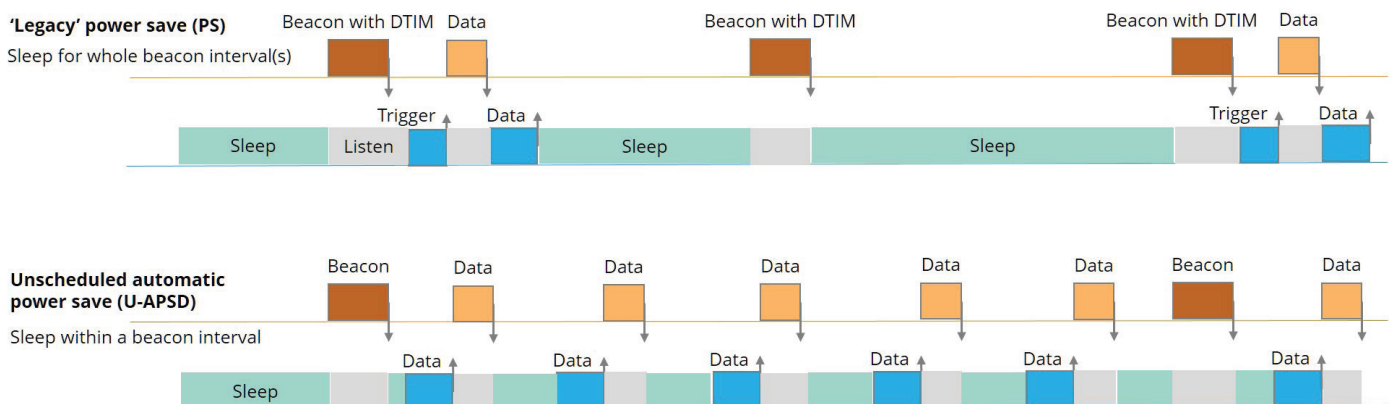
Figure 28: Power-save options before 802.11ax
